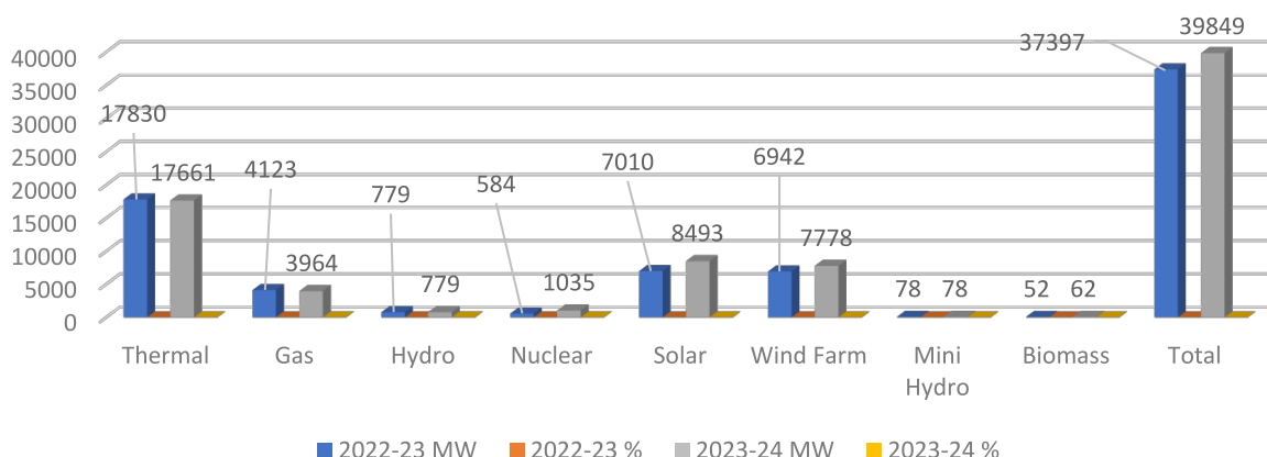
Installed Capacity (Fuel Wise) (MW)
